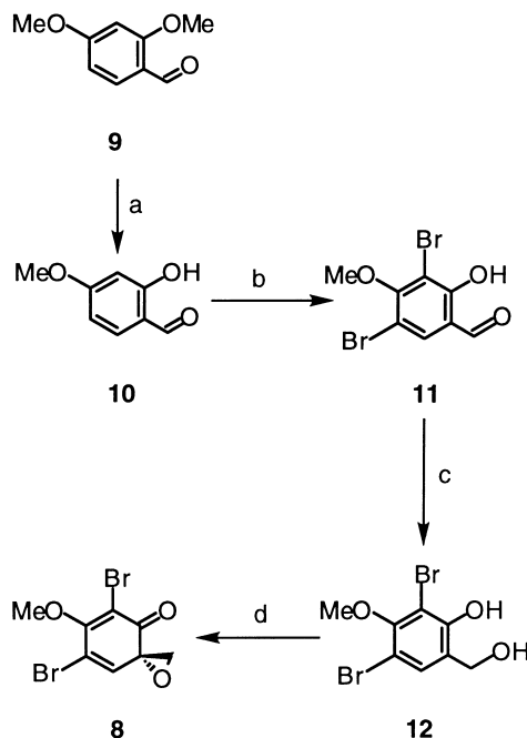
Scheme 2. Synthesis of the spiro -epoxy aeropylsinin analogue 8 ; (a) \text{BCl}_3 , \text{CH}_2\text{Cl}_2 , rt, 93%; (b) \text{Br}_2\text{-HBrpyridine} , pyridine, 65^\circ\text{C} , 75%; (c) \text{NaBH}_4 , THF, rt, 93%; (d) \text{NaIO}_4 , \text{HCl} , \text{H}_2\text{O} , THF, rt, 60%.
