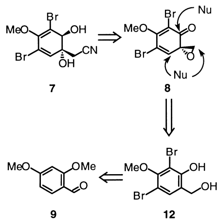
Scheme 1. Structure of aeropylsinin 7 and the spiro -epoxy analogue 8 ; retrosynthetic analyses of 7 and 8 .
