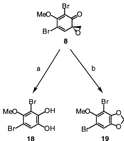
Scheme 3. Synthesis of the aeropylsinin analogues 18 and 19 ; (a) THF, 1 N HCl, 70 °C, 72%; (b) toluene, 60 °C, 78%.
